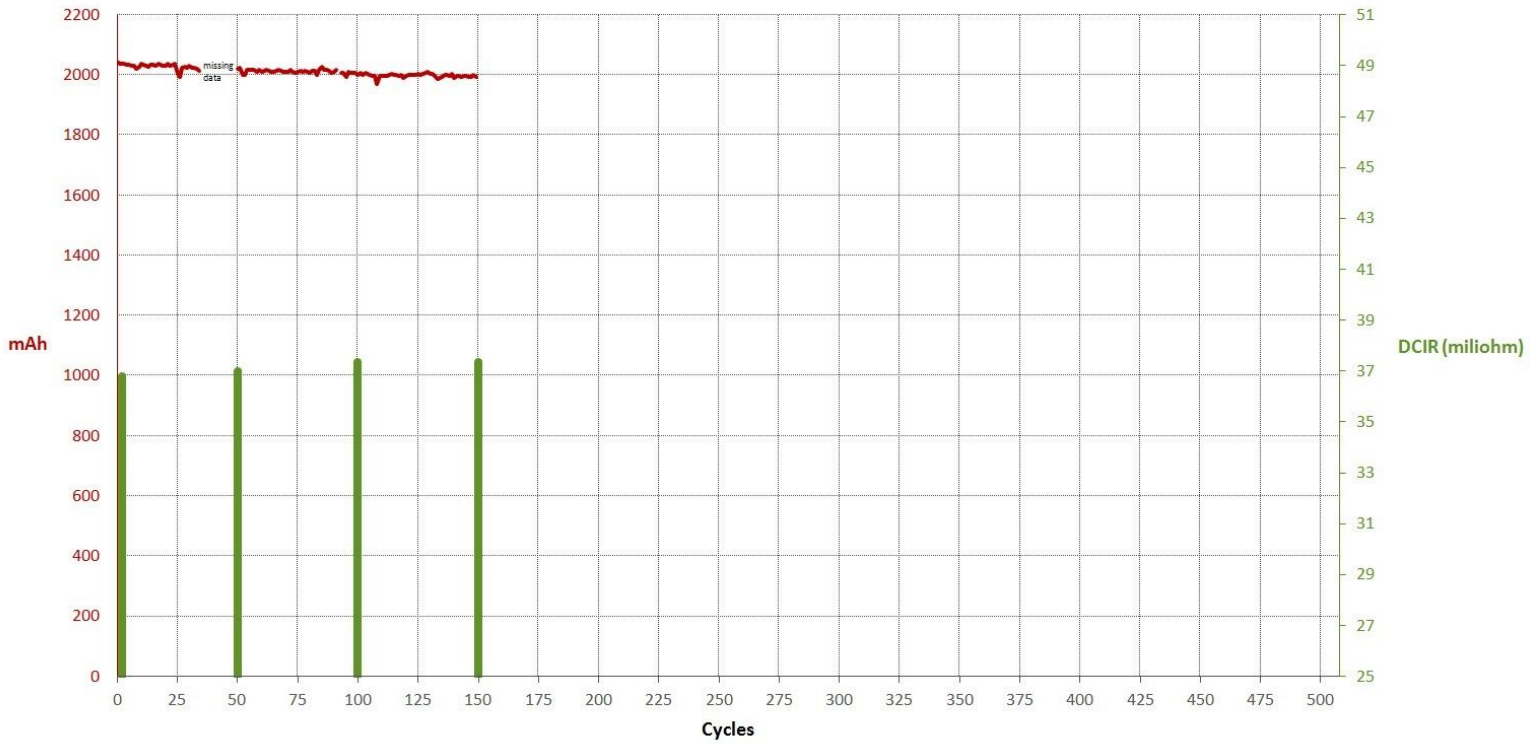
LG MJ1 150 cycles.jpg (172.53 KiB) Viewed 2419 times
